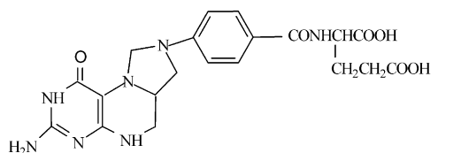
N 5 ,N 10 -methylenetetrahydrofolate
