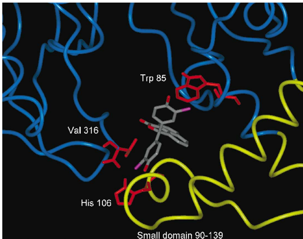
Figure 4. Detail of the X-ray crystal structure of the binary complex Lactobacillus casei TS-compound 8 . The small domain is colored in yellow.
