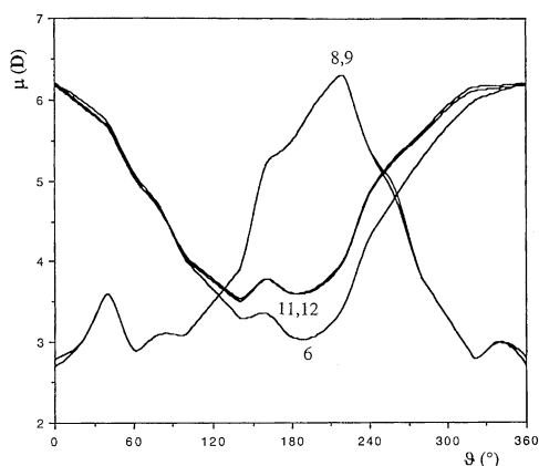
Figure 9. Dipole moment profiles for compounds 6 , 8 , 9 , 11 , 12 .
