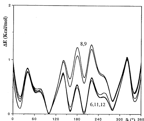
Figure 8. Rotational profile for compounds 6 , 8 , 9 , 11 , 12 . The solid line is obtained from interpolation of the calculation results every 20°, as described in Experimental.
