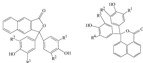
Figure 2. Phthalain and naphthalain derivatives. 4
