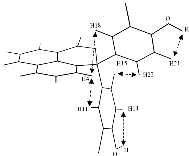
Figure 7. Compound 10 is reported with the conformation supported by ^1\text{H}/2\text{D} -NOESY spectrum at 170 K in acetone- d_6 (see Fig. 6). The protons referring to NOEs are indicated by arrows.
