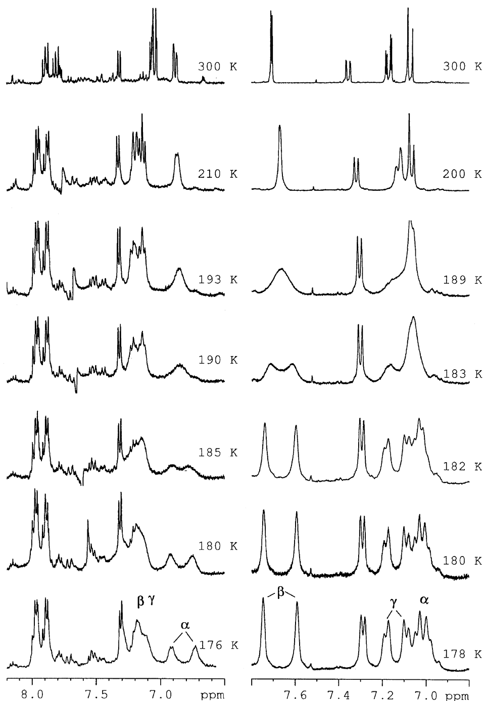
Figure 5. ^1\text{H} NMR spectra of compounds 7 (left panel) and 10 (right panel) in acetone- d_6 at different temperatures. The splitting protons are indicated as follows: \alpha = H14, \beta = H11, \gamma = H15. With decreasing temperature, the splitting of the proton signal of the phenol rings is evident.
