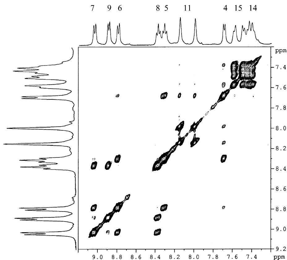
Figure 6. ^1\text{H}/2\text{D} -NOESY spectrum of compound 10 recorded at 170 K in acetone- d_6 using 200 ms of mixing time.
